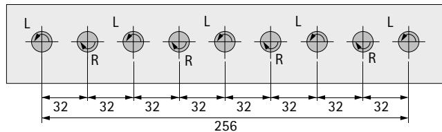
Drilling pattern
